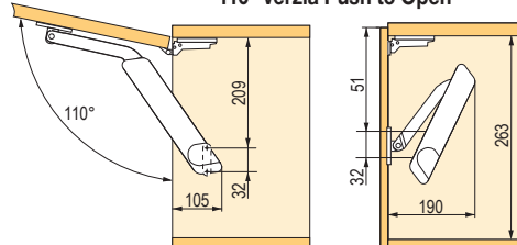
110° verzia Push-to-Open
