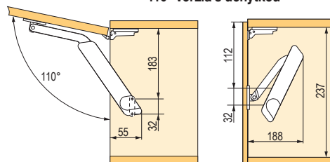
110° verzia Push-to-Open
