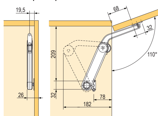
110° verzia push to open
