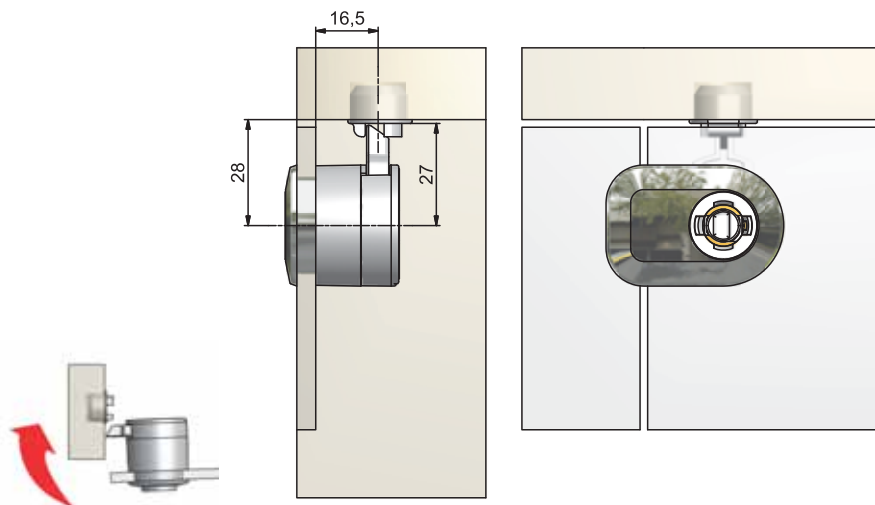
Glass door internally mounted Glastür innenliegend
