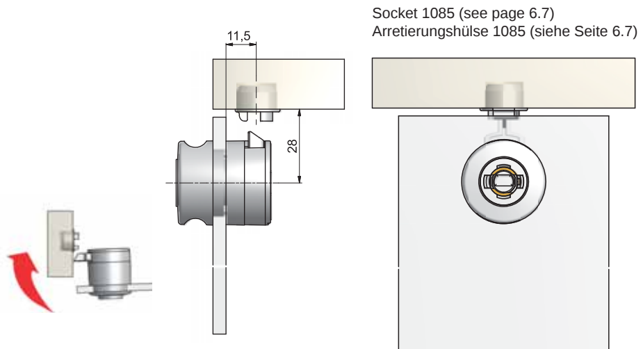
Glass door internally mounted Glastür innenliegend
