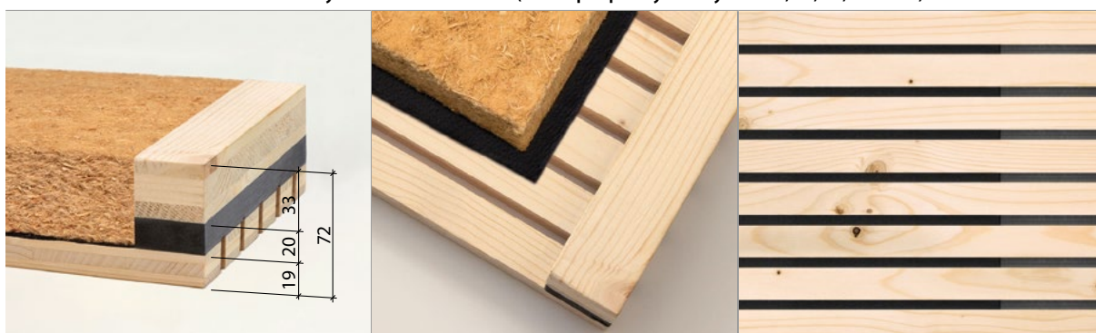
Svlak – SWP + MDF černý / Absorbér – Fibertex, Steico Flex
